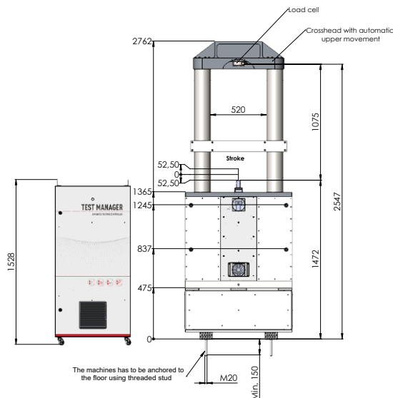
Ultra-high frequency test system - UHF
