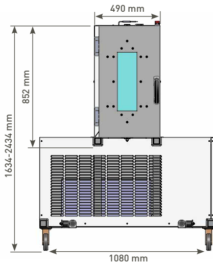
CC80SP - Dimensions
